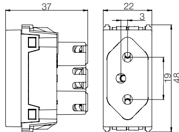
Tomada 2P+T-20 A
